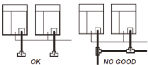
T-shape branching joint for liquid pipe
