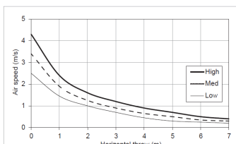
MMK-UP0121HP-E High wind: 4.3m/s Mid wind: 3.4m/s Low wind: 2.5m/s
