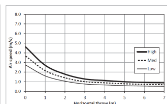
MMK-UP0151HP-E High wind: 4.6m/s Mid wind: 3.7m/s Low wind: 2.8m/s
